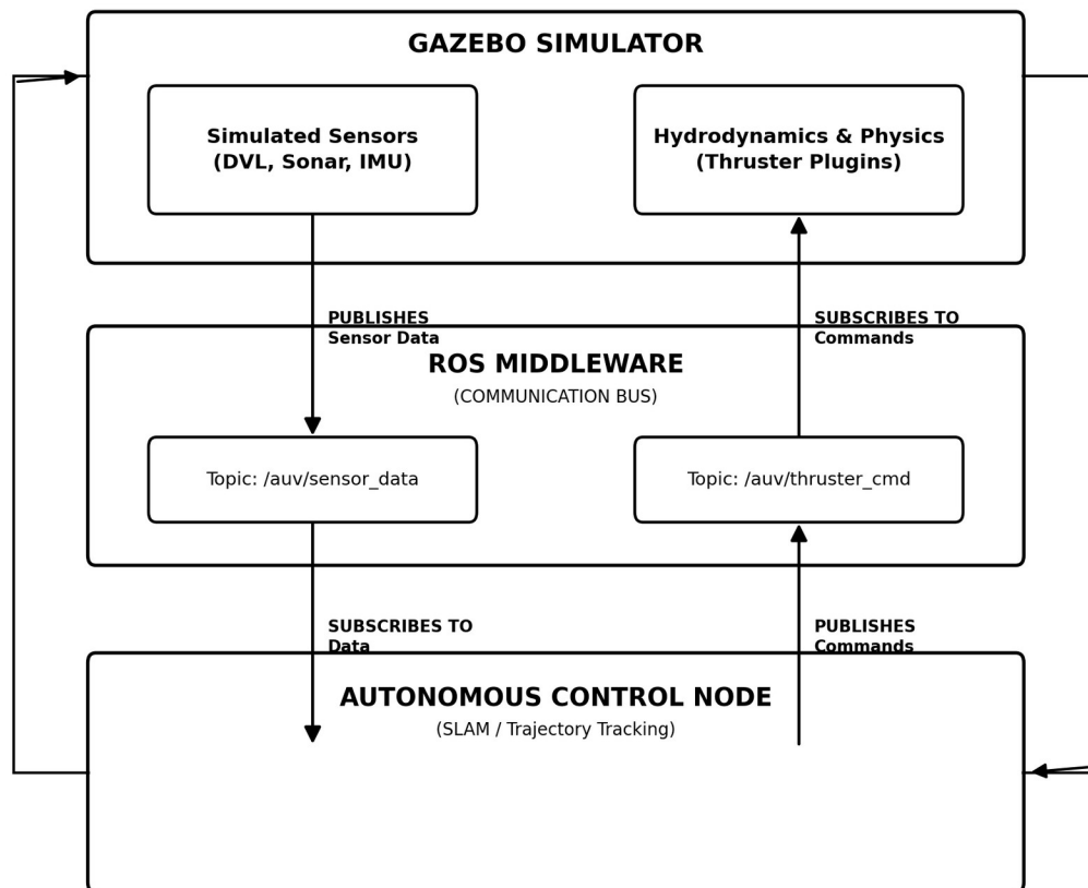
Figure 1: Publish/Subscribe data flow between the Gazebo Simulator, the ROS middleware, and the Autonomous Control Node.
